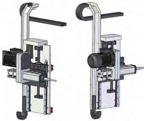
Gantry slide Horizontal left CP.HI
